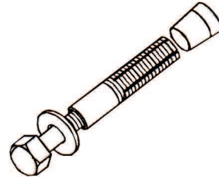
Chumbadro CB - Rosca Interna
